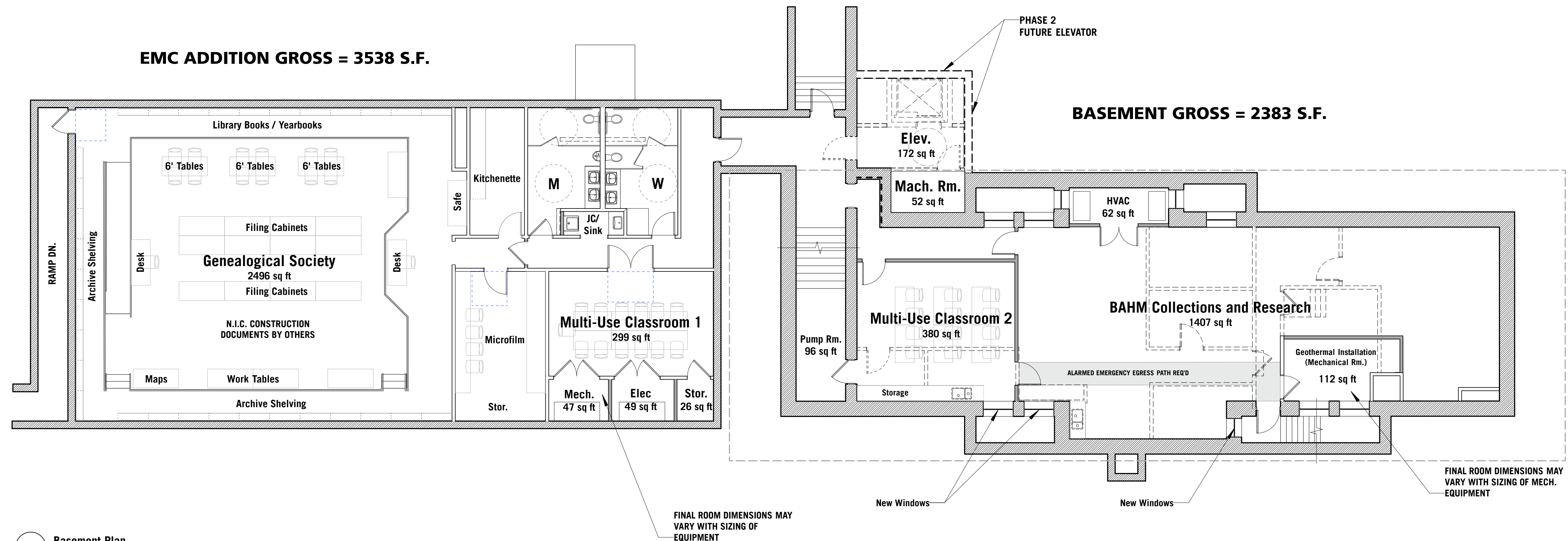
1 Basement Plan Scale: 1/8" = 1'-0"
